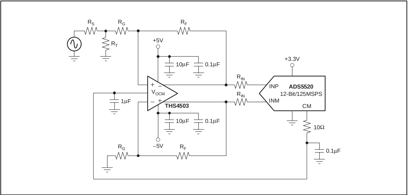
Figure 7. Using the THS4503 with the ADS5520
