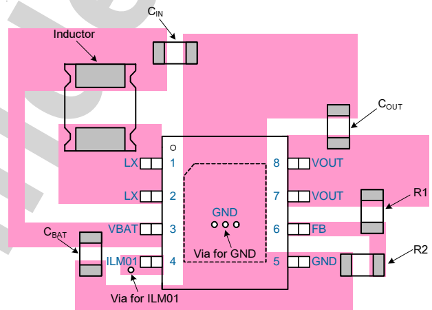
Figure 1. PSOP - 8L Layout Reference
