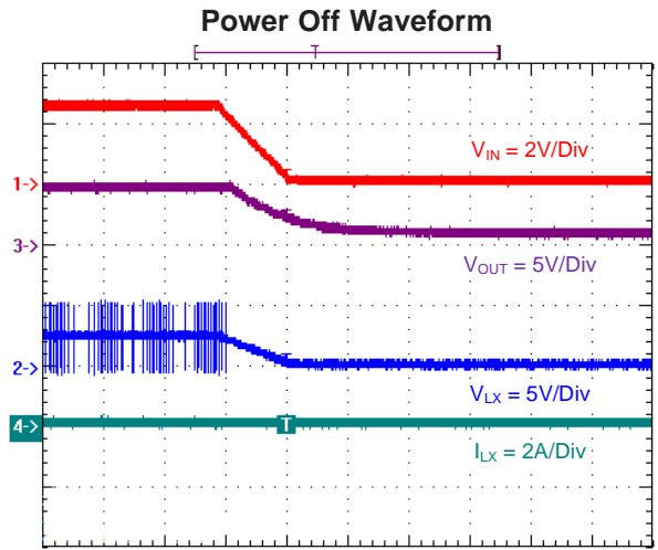
Time (20ms/Div) V_{IN} = 2.5V, I_{OUT} = 0A
