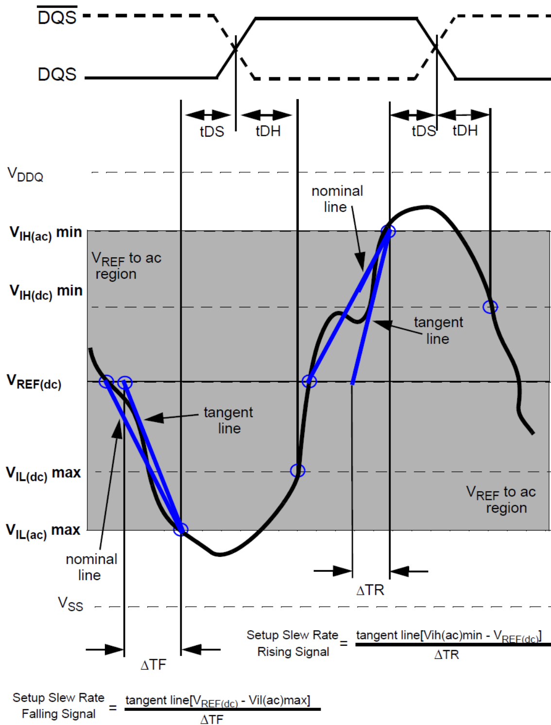
Illustration of tangent line for tDS (differential DQS, \overline{DQS} )
