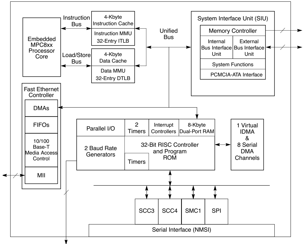
Figure 1-1. MPC852T Block Diagram
