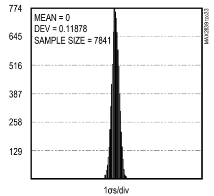
HISTOGRAM: RX PHASE IMBALANCE
