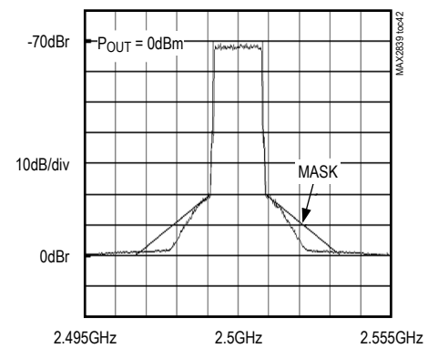
TX OUTPUT SPECTRUM (10MHz CHANNEL BANDWIDTH, 16 QAM FUSC)
