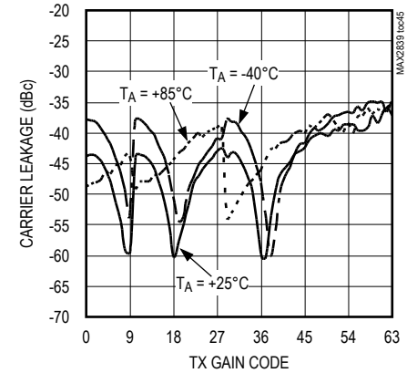
TX CARRIER LEAKAGE vs. GAIN SETTING
