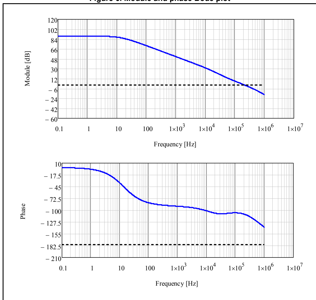
Figure 6. Module and phase Bode plot
