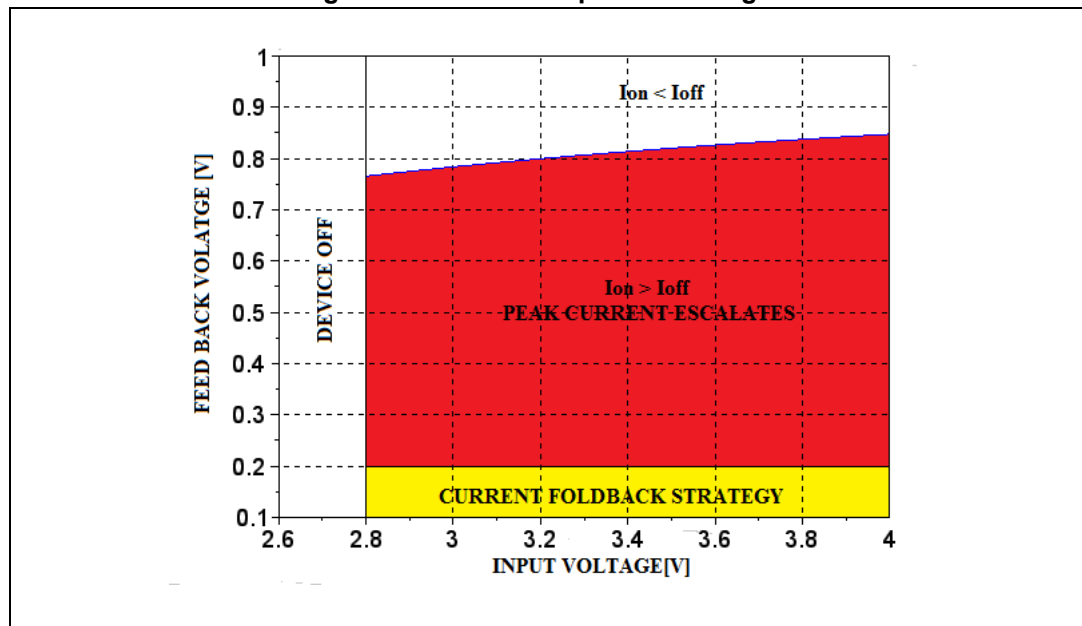
Figure 7. Overcurrent protection region
