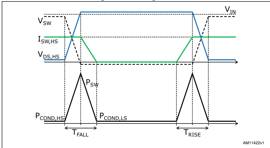
Figure 8. Switching losses
