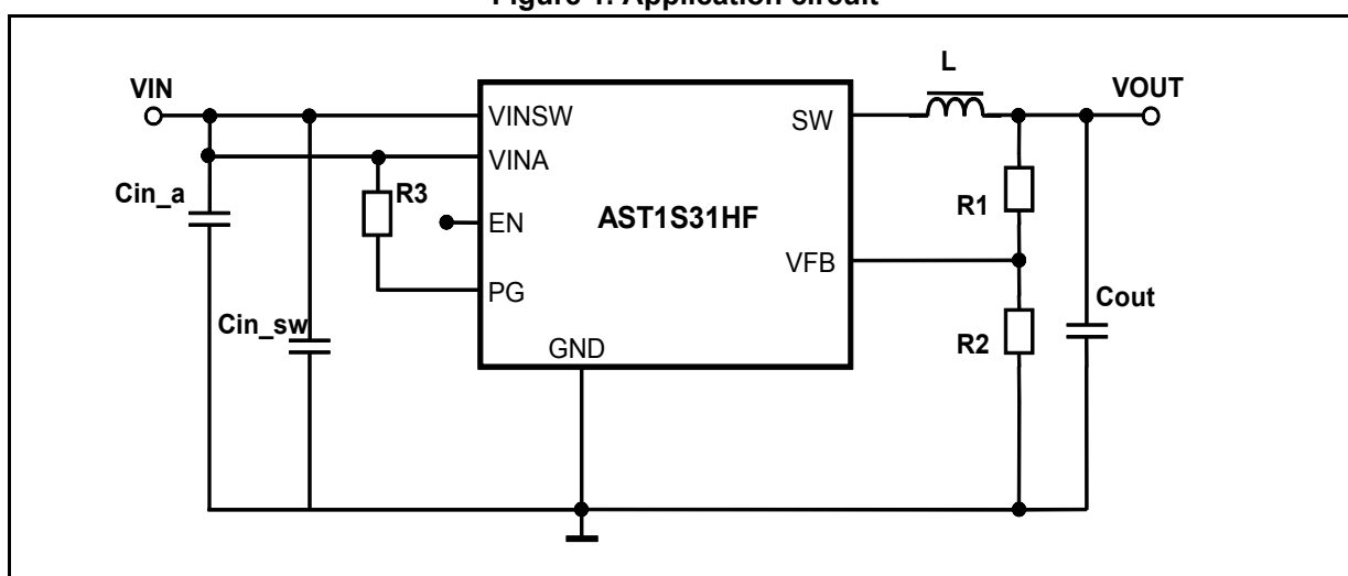
Figure 1. Application circuit
