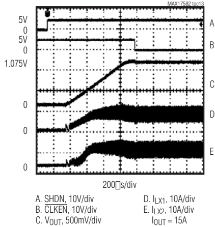
SOFT-START WAVEFORM (UP TO CLKEN)
