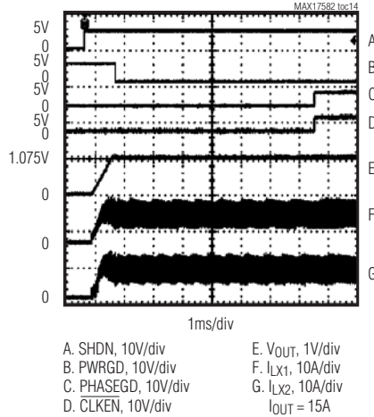
SOFT-START WAVEFORM (UP TO PWRGD)
