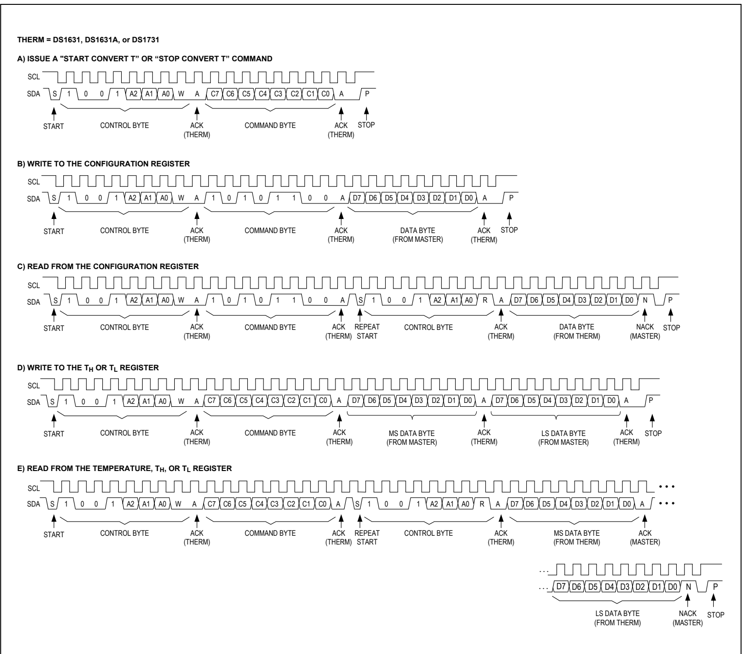
Figure 9. (a, b, c, d, e). 2-Wire Interface Timing
