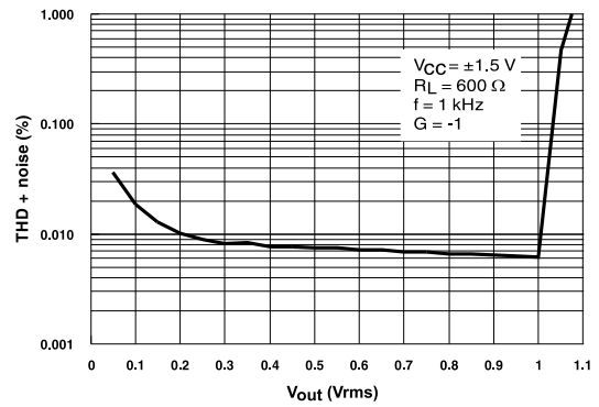
Figure 8. THD + noise vs. V out , R L = 600 Ω
