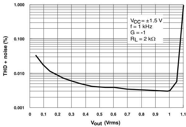
Figure 9. THD + noise vs. V out , R L = 2 kΩ
