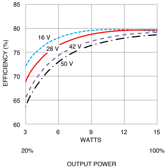
MFK283R3S EFFICIENCY
