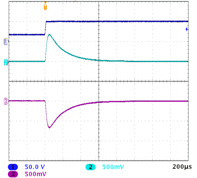
MFK2815D STEP LINE 16 - 50 VOLTS 50% LOAD
