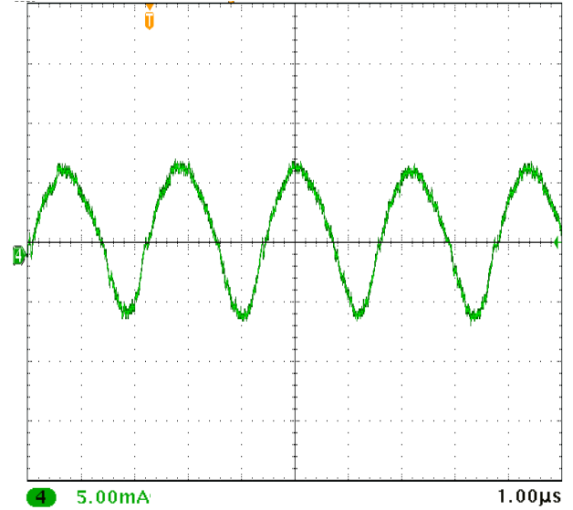
MFK2805S INPUT RIPPLE
