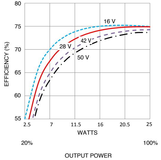
MFK282R5S EFFICIENCY
