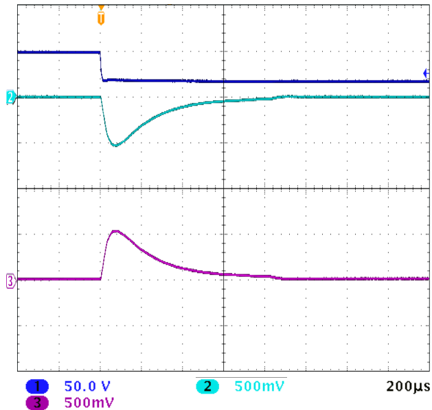
MFK2815D STEP LINE 50 - 16 VOLTS 50% LOAD
