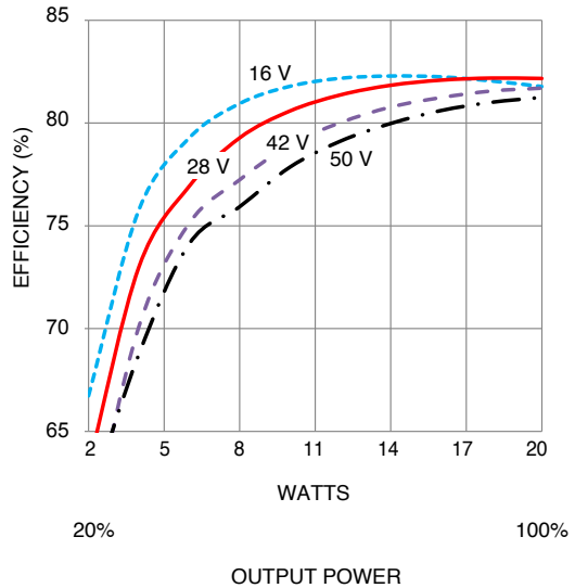
MFK2805S EFFICIENCY
