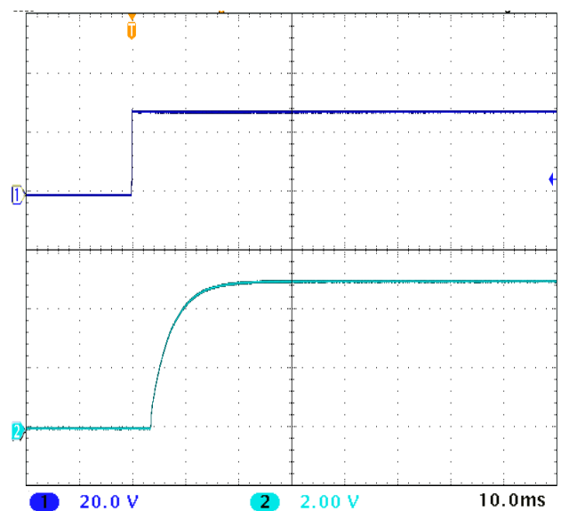
MFK2805S START-UP FULL LOAD
