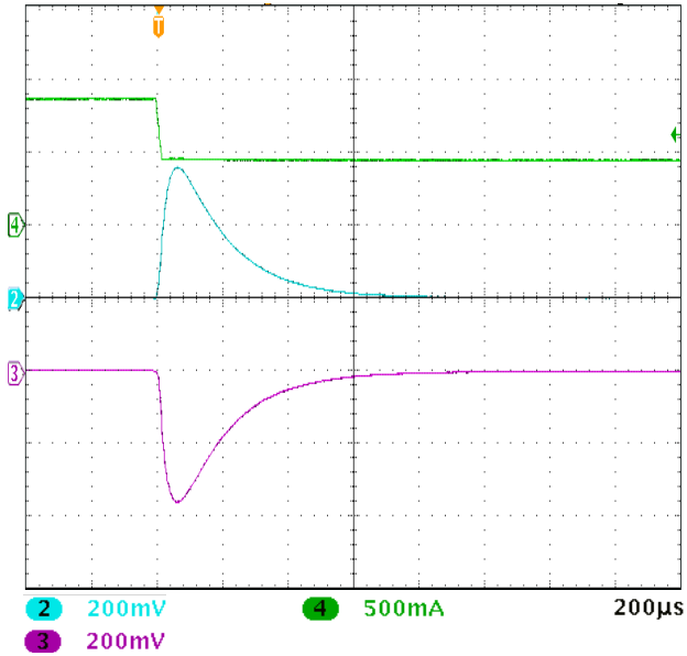
MFK2815D STEP LOAD 100% - 50%
