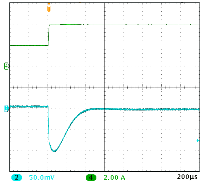
MFK2805S STEP LOAD 50% - 100%
