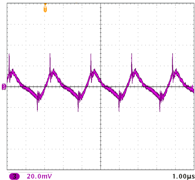
MFK2805S OUTPUT RIPPLE
