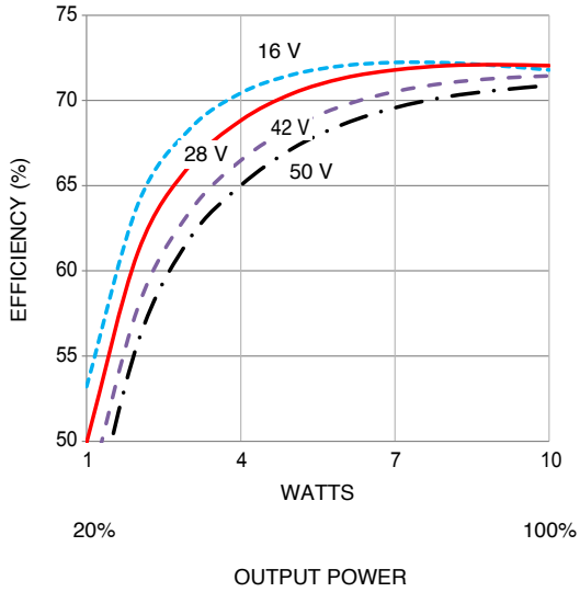
MFK281R8S EFFICIENCY
