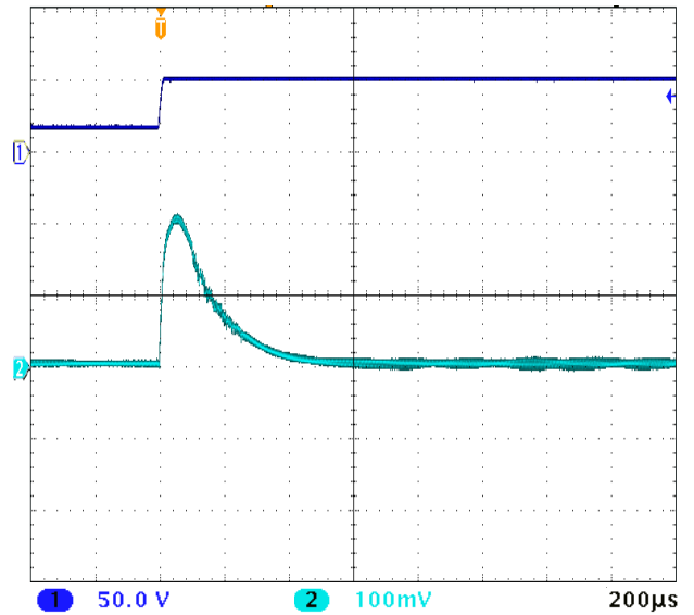
MFK2805S STEP LINE 16 - 50 VOLTS 50% LOAD
