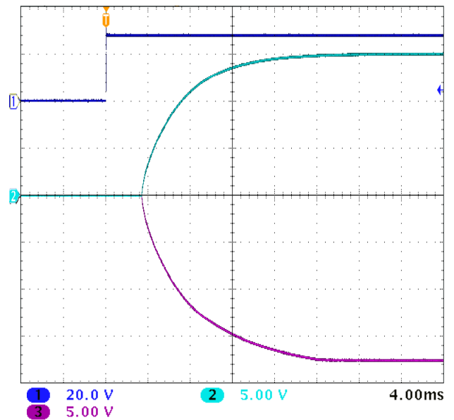
MFK2815D START-UP FULL LOAD
