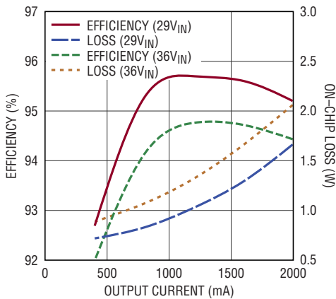
Efficiency
