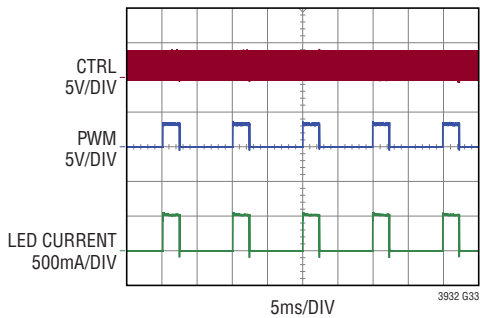
Digital PWM 25%
