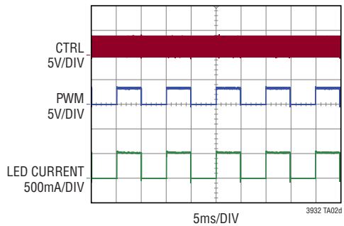
Digital PWM 50%
