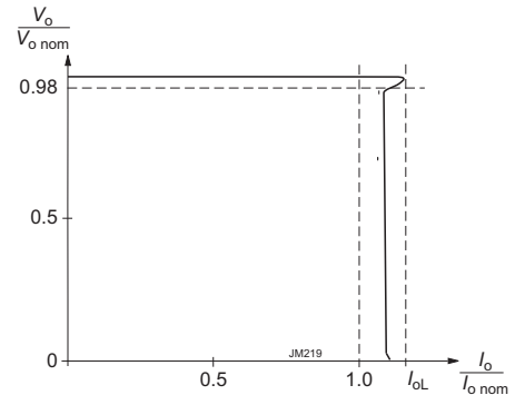
Fig. 6 Rectangular current limitation
