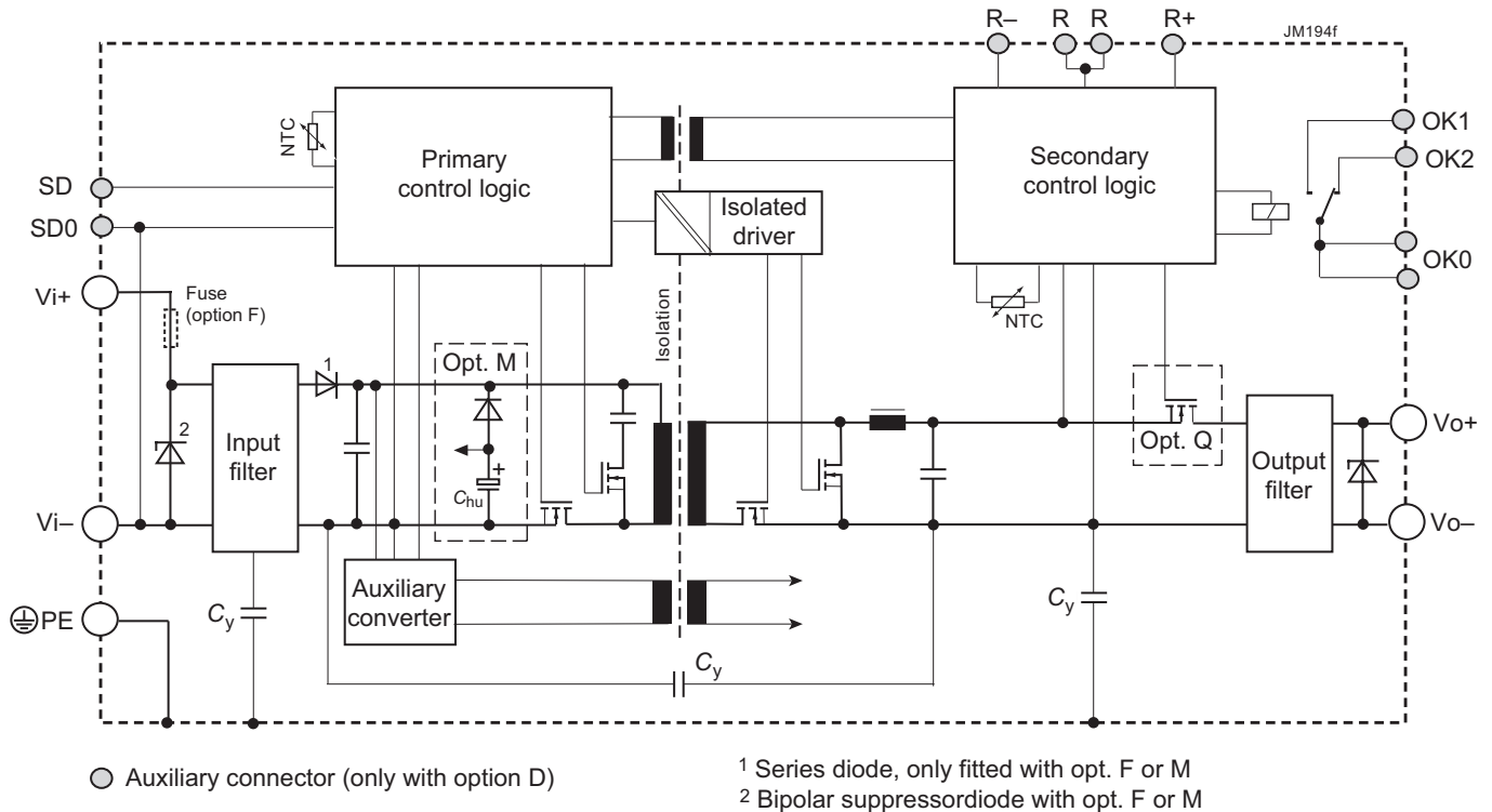
Fig. 1 Block diagram
