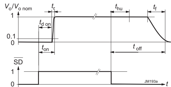
Fig. 8 Typical output response to the SD-signal. If option M is not fitted, t_{hu} = 0\ \text{ms} .
