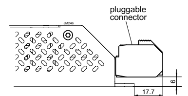
Fig. 12b Plugged connector for RCM300 with option K
