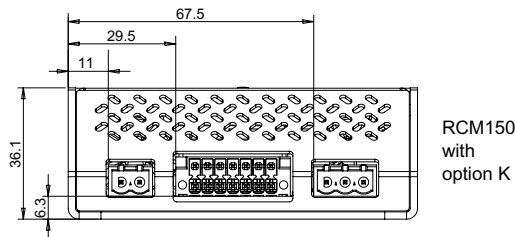
Fig. 11a Case of RCM150 (RCM01) weight approx. 520 g, Aluminum, EP-powder coated
