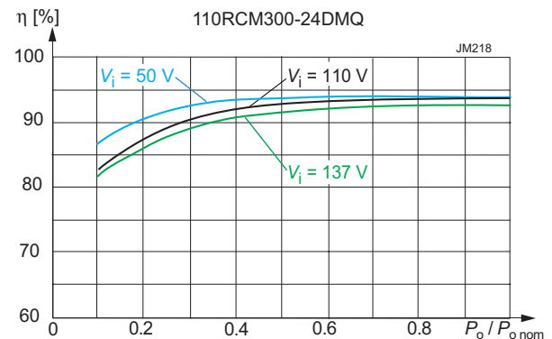
Fig. 3c Efficiency versus V_i and P_o (110RCM300-24DMQ)
