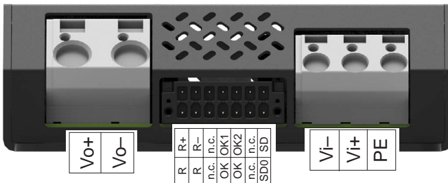
Fig. 14 Pin allocation of RCM300
