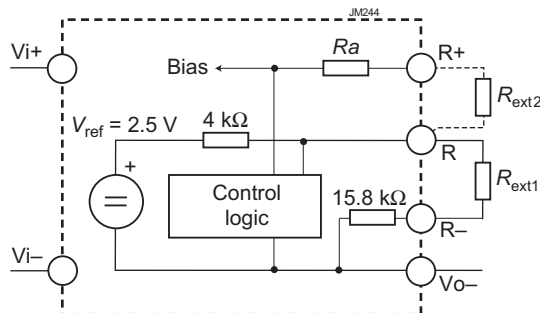
Fig. 7 Output voltage control via R-input
