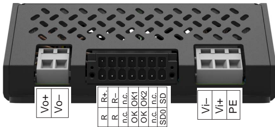
Fig. 13 Pin allocation of RCM150
