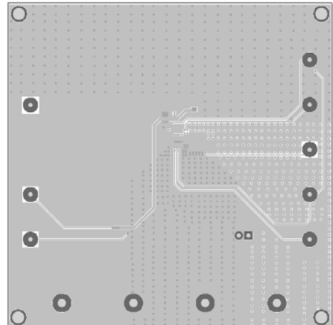
Figure 4: Inner 2 Layer
