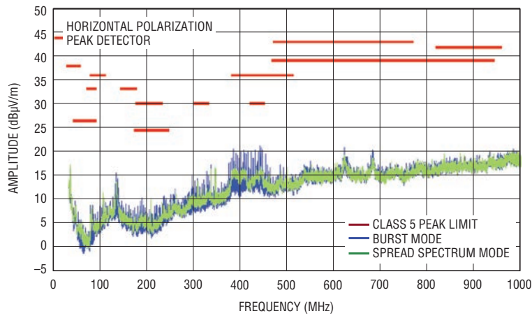
DC2202A DEMO BOARD (WITH EMI FILTER INSTALLED) 14V INPUT TO 5V OUTPUT AT 4A, f_{SW} = 2\text{MHz}
