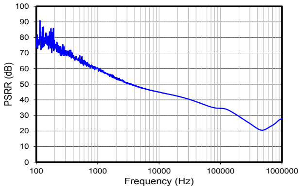
LDO2=1.8V, PSRR, Iout=30mA
