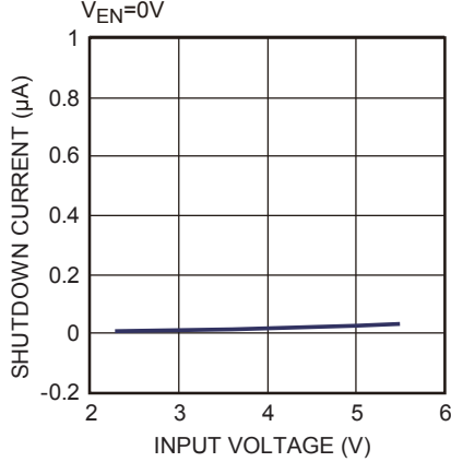
Shutdown Current vs. Input Voltage V EN =0V
