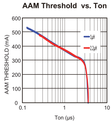
Figure 9: AAM Threshold Decreases with T_{ON} Increasing
