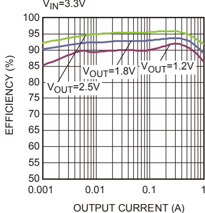
Efficiency vs. Output Current V IN =3.3V
