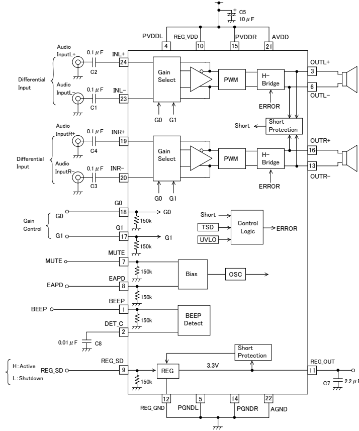
Differential input
