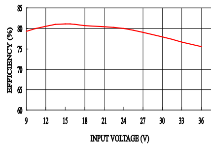
LANEUW2405R3 Efficiency vs Input Voltage
