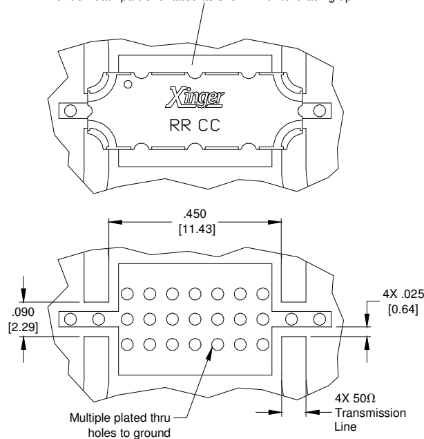
Dimensions Are in Inches [Millimeters] XEC24E3-03G Mounting Footprint
