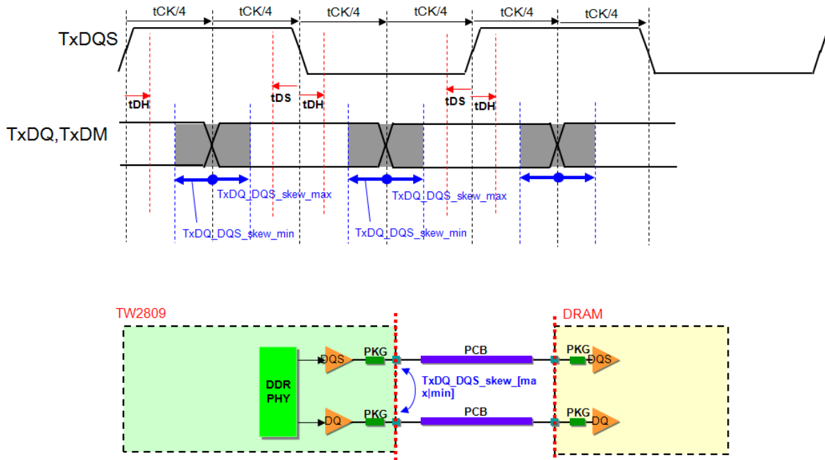
FIGURE 32. TXDQ-DQS TIMING
