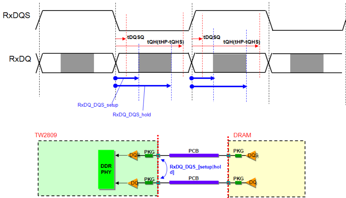
FIGURE 33. RXDQ-DQS TIMING
