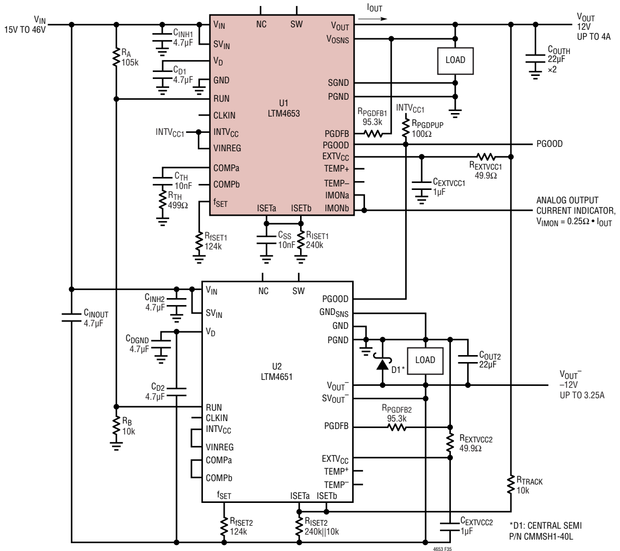
Figure 35. Concurrent ±12V Supply. See Figure 34 for Output Voltage Start-Up Waveforms
