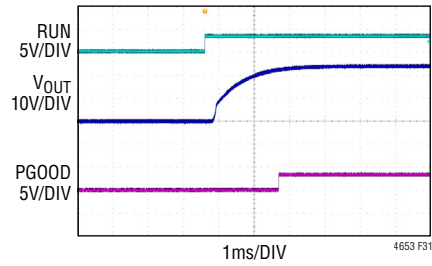
Figure 31. Start-Up Waveforms at 48V IN , Figure 30 Circuit
