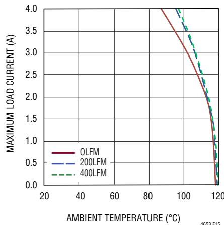
Figure 15. 12V to 1VOUT Derating Curve, with BGA Heat Sink
