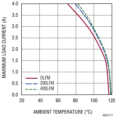
Figure 17. 12V to 5V OUT Derating Curve, No Heat Sink
