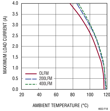
Figure 18. 24V to 5V OUT Derating Curve, No Heat Sink
