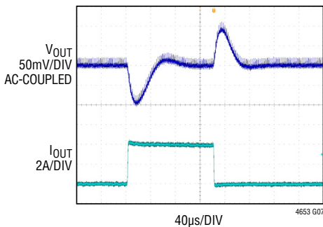
FIGURE 30 CIRCUIT, 48V IN , C_{INH} = C_D = 4.7\mu\text{F} , C_{OUT} = 2 \times 100\mu\text{F} , R_{FSET} = \text{N/A} , R_{ISET} = 66.5\text{k}\Omega , C_{TH} = 10\text{nF} , R_{TH} = 604\Omega , R_{EXTVCC} = \text{N/A} , C_{EXTVCC} = \text{N/A} , 2A to 4A LOAD STEP AT 2A/ \mu\text{s}
