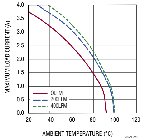
Figure 25. 48V to 24V OUT Derating Curve, No Heat Sink
