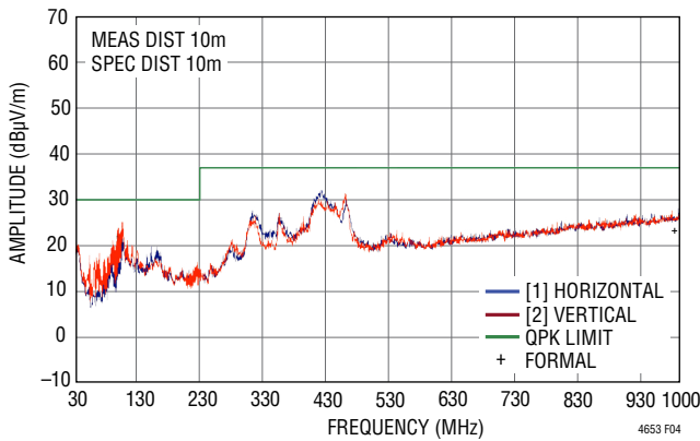
Figure 4. Radiated Emissions Scan of the LTM4653. Producing 24V OUT at 4A, from 29.5V IN . DC2327A Hardware. f SW = 1.2MHz. Measured in a 10m Chamber. Peak Detect Method
