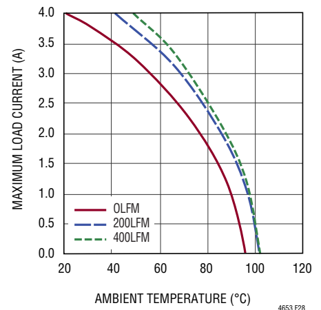
Figure 28. 48V to 24V OUT Derating Curve, with BGA Heat Sink
