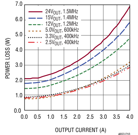
Figure 10. 48VIN Power Loss Curve
