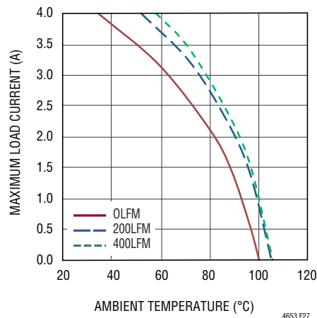
Figure 27. 48V to 15V OUT Derating Curve, with BGA Heat Sink
