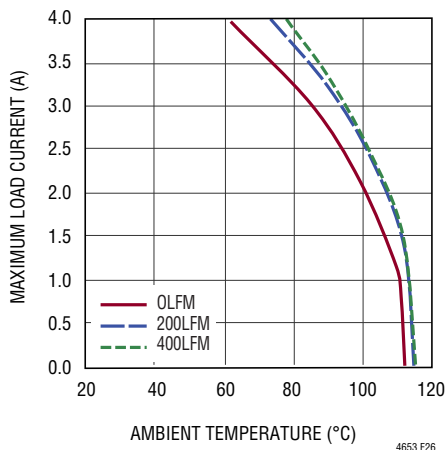
Figure 26. 24V to 15V OUT Derating Curve, with BGA Heat Sink
