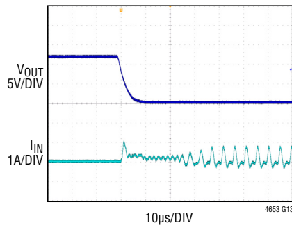
FIGURE 30 CIRCUIT, 48\text{V}_{\text{IN}} , C_{\text{INH}} = C_{\text{D}} = 4.7\mu\text{F} , C_{\text{OUT}} = 2 \times 22\mu\text{F} , R_{\text{ISET}} = 124\text{k} , R_{\text{ISET}} = 240\text{k}\Omega , R_{\text{PGDFB}} = 95.3\text{k}\Omega , C_{\text{TH}} = 10\text{nF} , R_{\text{TH}} = 562\Omega , R_{\text{EXTVCC}} = 49.9\Omega , C_{\text{EXTVCC}} = 1\mu\text{F} , NO LOAD PRIOR TO APPLICATION OF OUTPUT SHORT-CIRCUIT
