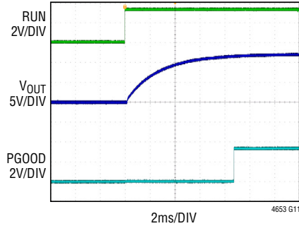
FIGURE 30 CIRCUIT, 48\text{V}_{\text{IN}} , C_{\text{INH}} = C_{\text{D}} = 4.7\mu\text{F} , C_{\text{OUT}} = 2 \times 22\mu\text{F} , R_{\text{ISET}} = 124\text{k} , R_{\text{ISET}} = 240\text{k}\Omega , R_{\text{PGDFB}} = 95.3\text{k}\Omega , C_{\text{TH}} = 10\text{nF} , R_{\text{TH}} = 562\Omega , R_{\text{EXTVCC}} = 49.9\Omega , C_{\text{EXTVCC}} = 1\mu\text{F} , 3\Omega RESISTIVE LOAD
