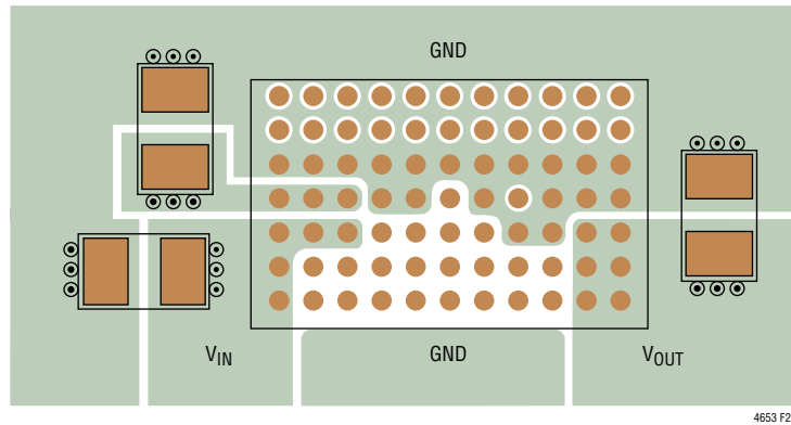
Figure 29. Recommend PCB Layout, Package Top View
