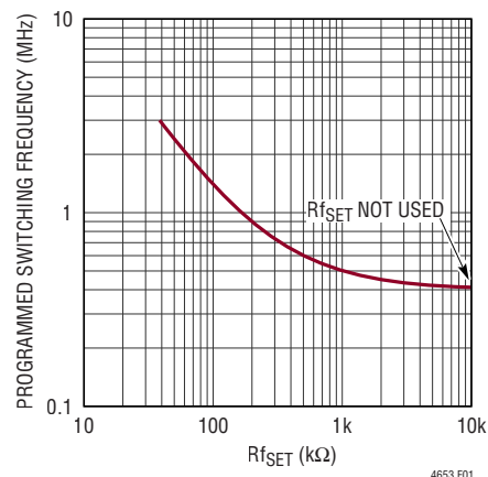
Figure 1. Relationship Between R_{\text{fSET}} and Target f_{\text{sw}}
