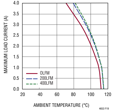
Figure 19. 48V to 5V OUT Derating Curve, No Heat Sink
