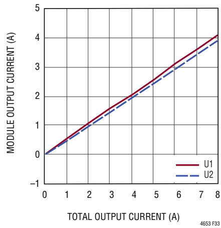
Figure 33. Current Sharing Performance of LTM4653s in Figure 32 Circuit
