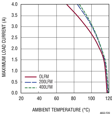
Figure 20. 12V to 5V OUT Derating Curve, with BGA Heat Sink
