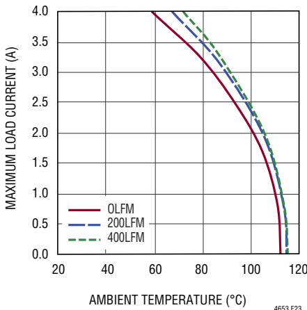
Figure 23. 24V to 15V OUT Derating Curve, No Heat Sink
