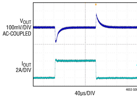
FIGURE 30 CIRCUIT, 48V IN , C_{INH} = C_D = 4.7\mu\text{F} , C_{OUT} = 2 \times 22\mu\text{F} , R_{FSET} = 124\text{k} , R_{ISET} = 240\text{k}\Omega , C_{TH} = 10\text{nF} , R_{TH} = 562\Omega , R_{EXTVCC} = 49.9\Omega , C_{EXTVCC} = 1\mu\text{F} , 2A to 4A LOAD STEP AT 2A/ \mu\text{s}
