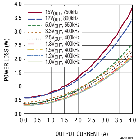
Figure 9. 24VIN Power Loss Curve
