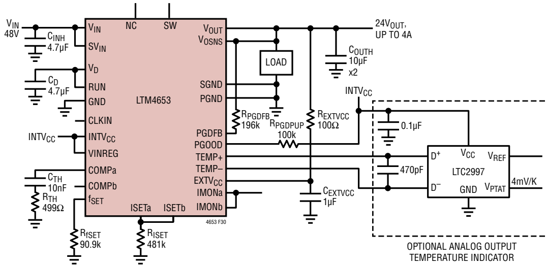
Figure 30. 4A, 24V Output DC/DC μModule Regulator
