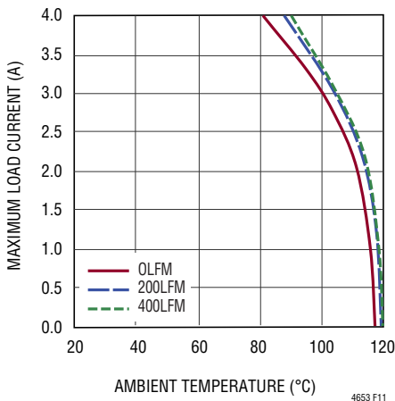
Figure 11. 5V to 1VOUT Derating Curve, No Heat Sink
