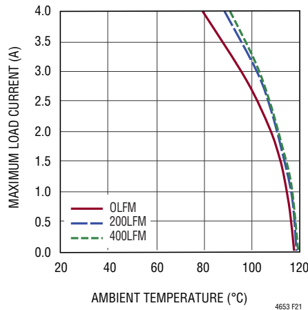
Figure 21. 24V to 5V OUT Derating Curve, with BGA Heat Sink
