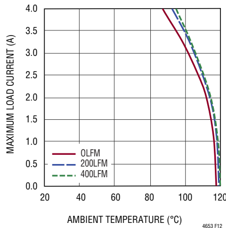
Figure 12. 12V to 1VOUT Derating Curve, No Heat Sink
