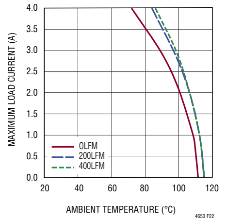
Figure 22. 48V to 5V OUT Derating Curve, with BGA Heat Sink
