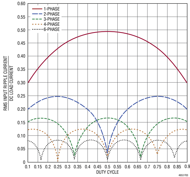
Figure 3. Normalized Input RMS Ripple Current vs Duty Cycle for One to Six LTM4653s (Phases)
