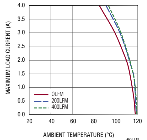
Figure 13. 24V to 1VOUT Derating Curve, No Heat Sink
