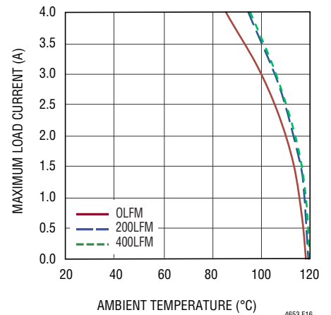
Figure 16. 24V to 1VOUT Derating Curve, with BGA Heat Sink
