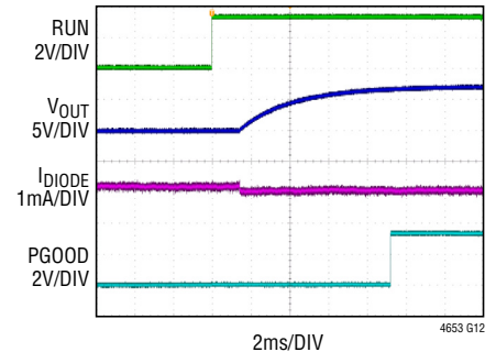
FIGURE 30 CIRCUIT, 48\text{V}_{\text{IN}} , C_{\text{INH}} = C_{\text{D}} = 4.7\mu\text{F} , C_{\text{OUT}} = 2 \times 22\mu\text{F} , R_{\text{ISET}} = 124\text{k} , R_{\text{ISET}} = 240\text{k}\Omega , R_{\text{PGDFB}} = 95.3\text{k}\Omega , C_{\text{TH}} = 10\text{nF} , R_{\text{TH}} = 562\Omega , R_{\text{EXTVCC}} = 49.9\Omega , C_{\text{EXTVCC}} = 1\mu\text{F} , V_{\text{OUT}} PRE-BIASED TO 5V THROUGH 1N4148 DIODE
