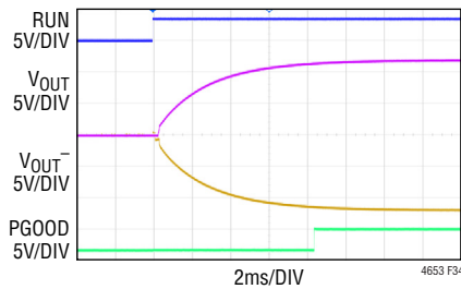
Figure 34. Concurrent \pm 12V Supply, Output Voltage Start-Up Waveforms, Figure 35 Circuit
