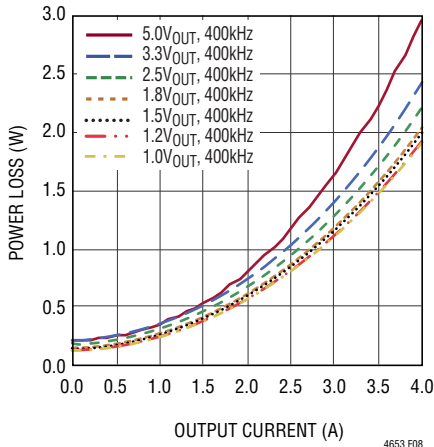
Figure 8. 12VIN Power Loss Curve
