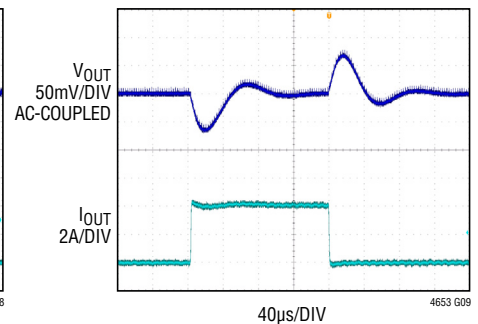
FIGURE 30 CIRCUIT, 24V IN , C_{INH} = C_D = 4.7\mu\text{F} , C_{OUT} = 3 \times 100\mu\text{F} , R_{FSET} = \text{N/A} , R_{ISET} = 20\text{k}\Omega , C_{TH} = 6.8\text{nF} , R_{TH} = 681\Omega , R_{EXTVCC} = \text{N/A} , C_{EXTVCC} = \text{N/A} , 2A to 4A LOAD STEP AT 2A/ \mu\text{s}
