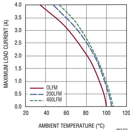
Figure 24. 48V to 15V OUT Derating Curve, No Heat Sink
