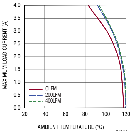
Figure 14. 5V to 1VOUT Derating Curve, with BGA Heat Sink
