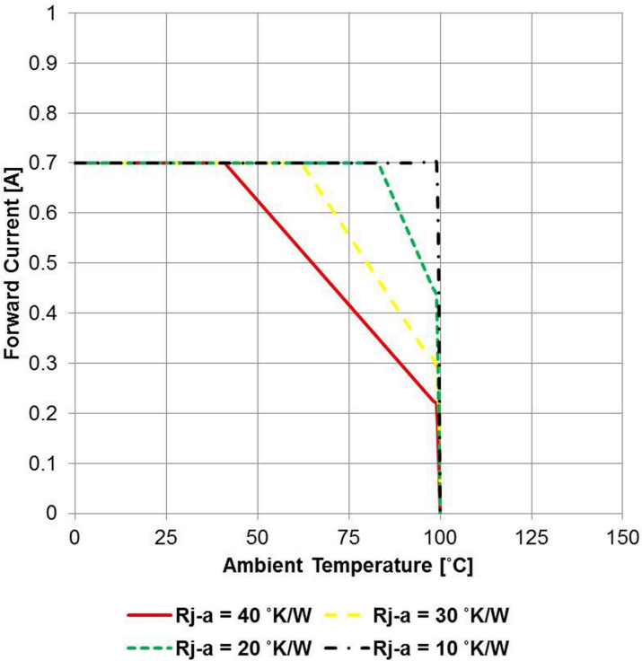
F7 Derating Curve:
