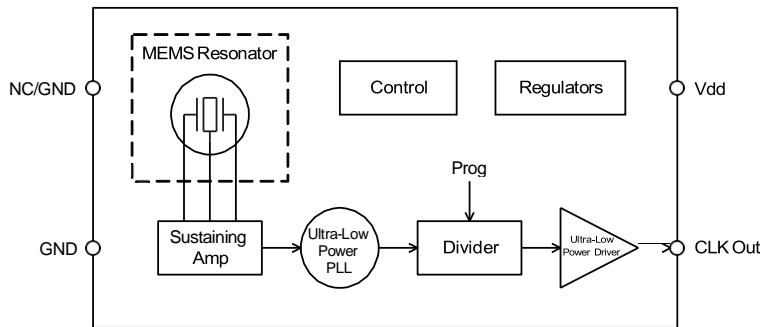
Figure 3. SIT1630 Block Diagram
