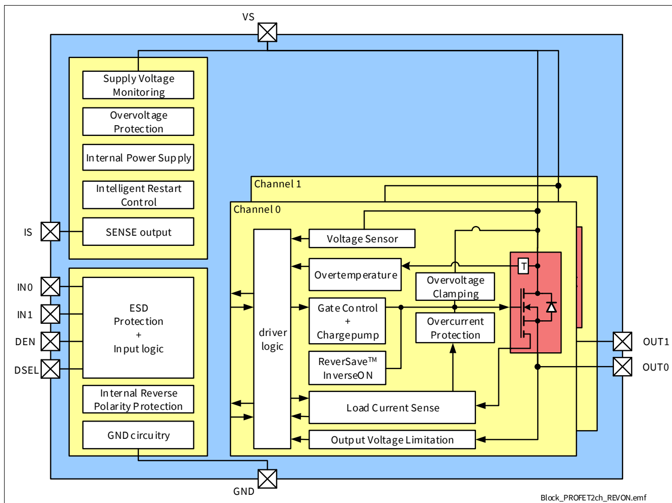
Figure 2 Block Diagram of BTS7040-2EPA
