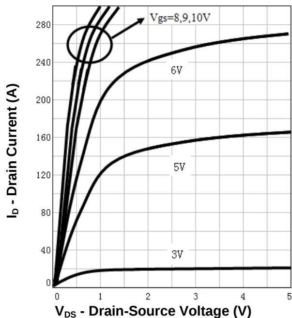
Output Characteristics
