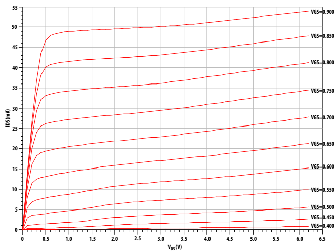
Figure 1. Typical I-V Curves. (VGS=0.05 V per step)
