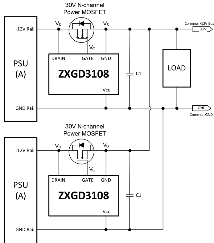
The focus application of the ZXGD3108 OR'ing Controller is for Redundant Low-Side -12V Power Supply Rail.
