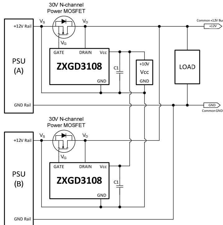
Example of the ZXGD3108 OR'ing Controller in a Redundant High-Side +12V Power Supply Rail with the addition of a Vcc Supply.
