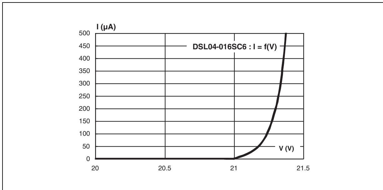
Figure 4. I / V characteristics (typical values)
