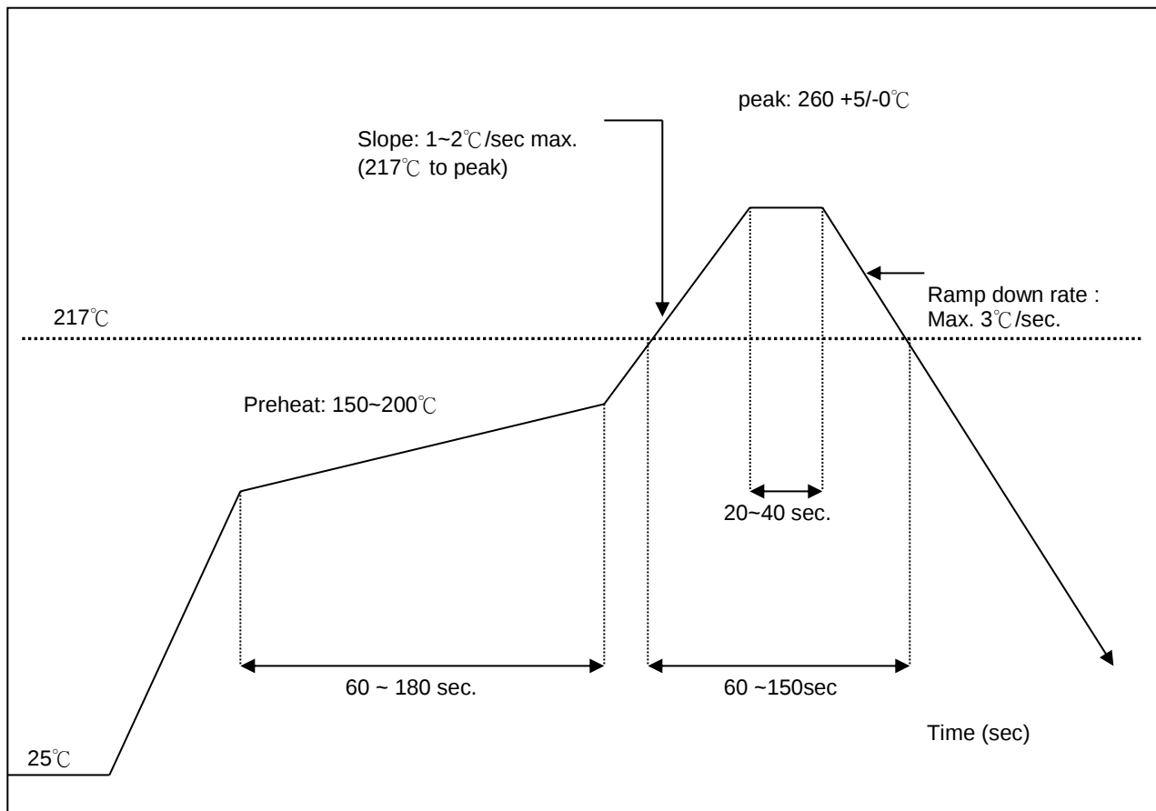
FIGURE 7-5: REFLOW PROFILE
