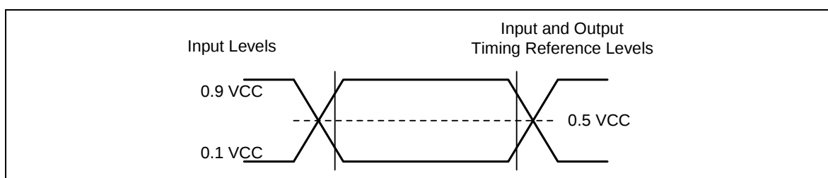
Figure 59. AC Measurement I/O Waveform
