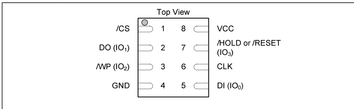
Figure 1b. W25Q32JV Pad Assignments, 8-pad WSON 6x5-mm (Package Code ZP)
