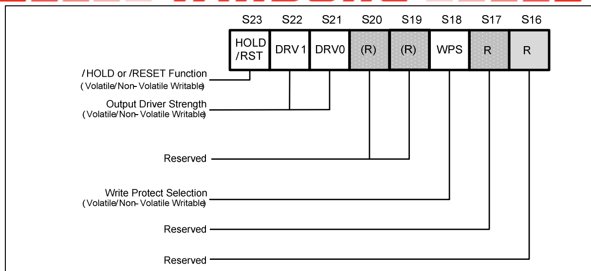
Figure 4c. Status Register-3
