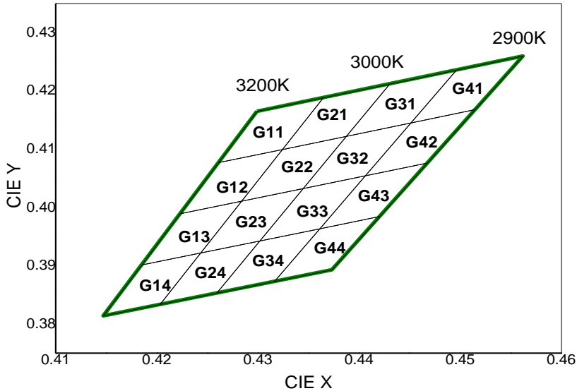
CIE Chromaticity Diagram (Warm white)
