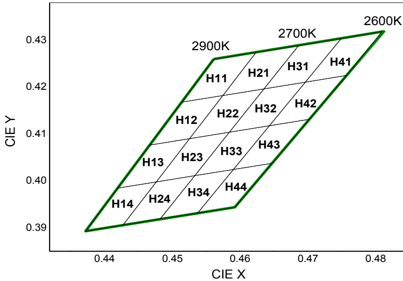
CIE Chromaticity Diagram (Warm white)
