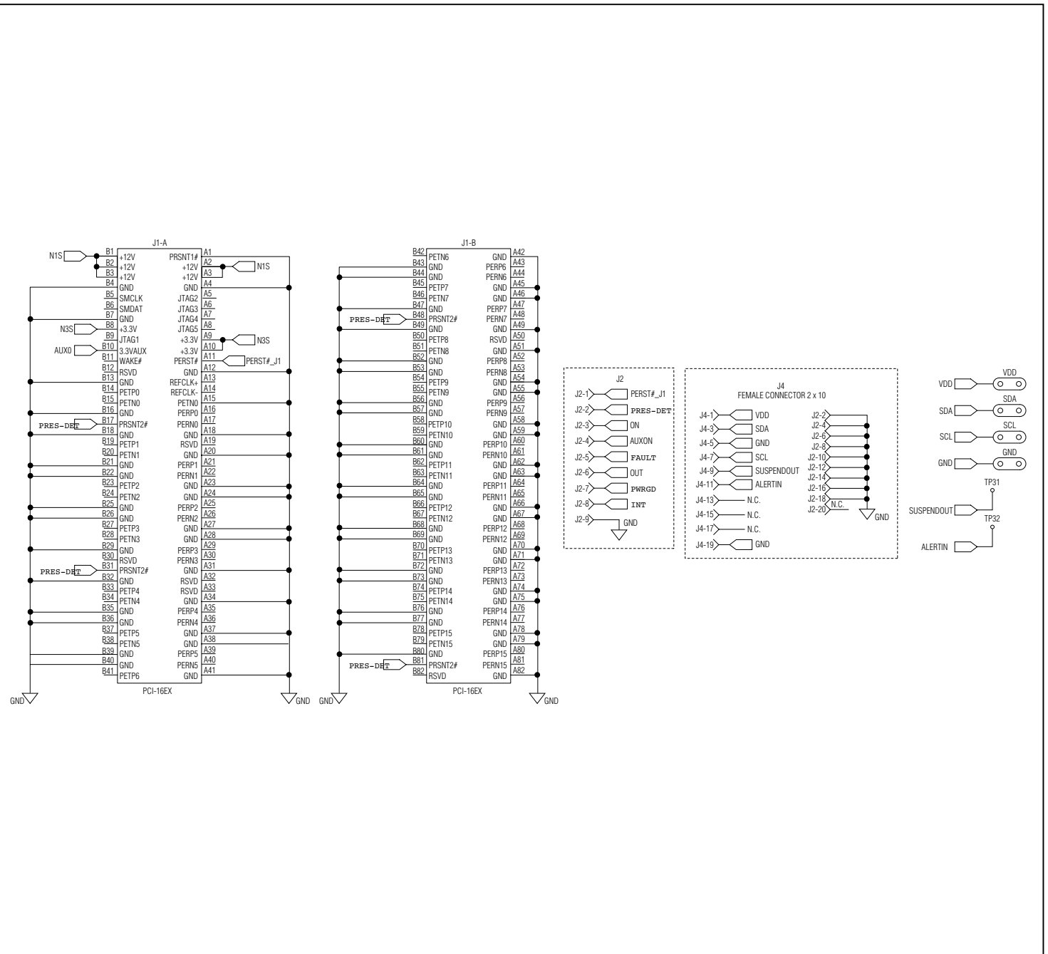
Figure 4. MAX5954L EV Kit Schematic, PCI Express X16 Connectors
