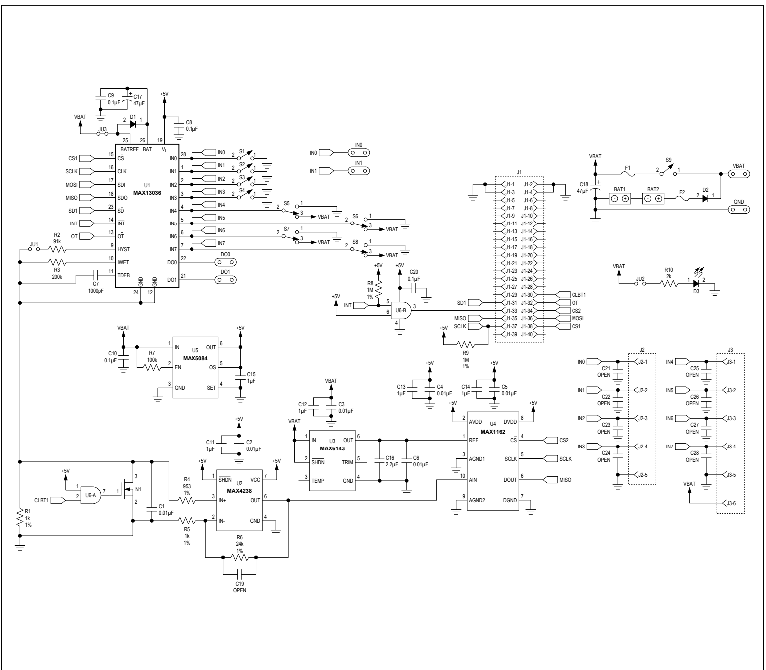
Figure 2. MAX13036 EV Kit Schematic
