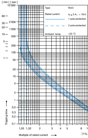
Tripping characteristics I_n \geq 3... < 18 \text{ A}
