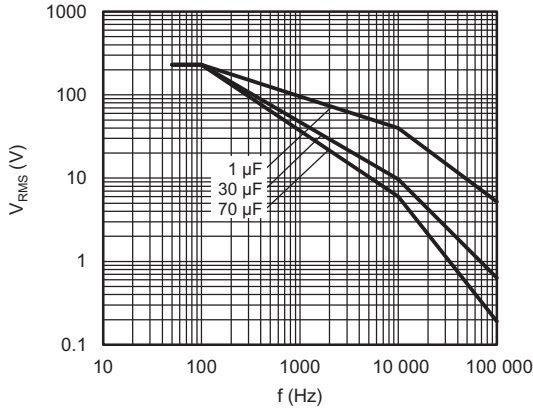
Maximum RMS voltage as function of frequency T_{amb} \leq 85\text{ }^{\circ}\text{C} ; U_n = 230\text{ V}_{AC}
