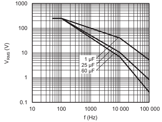
Maximum RMS voltage as function of frequency T_{amb} \leq 85\text{ }^{\circ}\text{C} ; U_n = 250\text{ V}_{AC}
