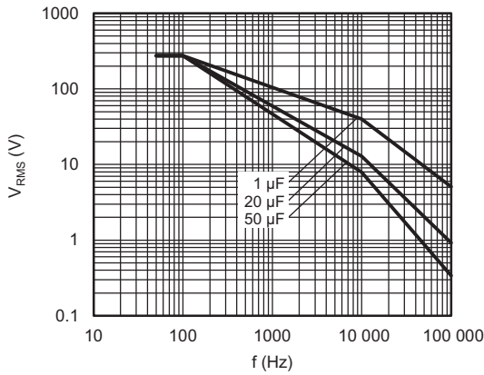
Maximum RMS voltage as function of frequency T_{amb} \leq 85\text{ }^{\circ}\text{C} ; U_n = 275\text{ V}_{AC}
