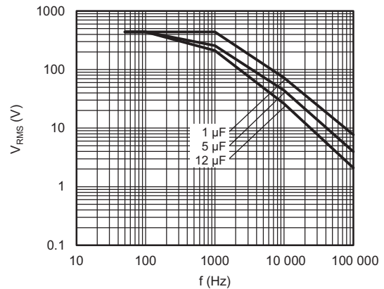
Maximum RMS voltage as function of frequency T_{amb} \leq 85\text{ }^{\circ}\text{C} ; U_n = 440\text{ V}_{AC}
