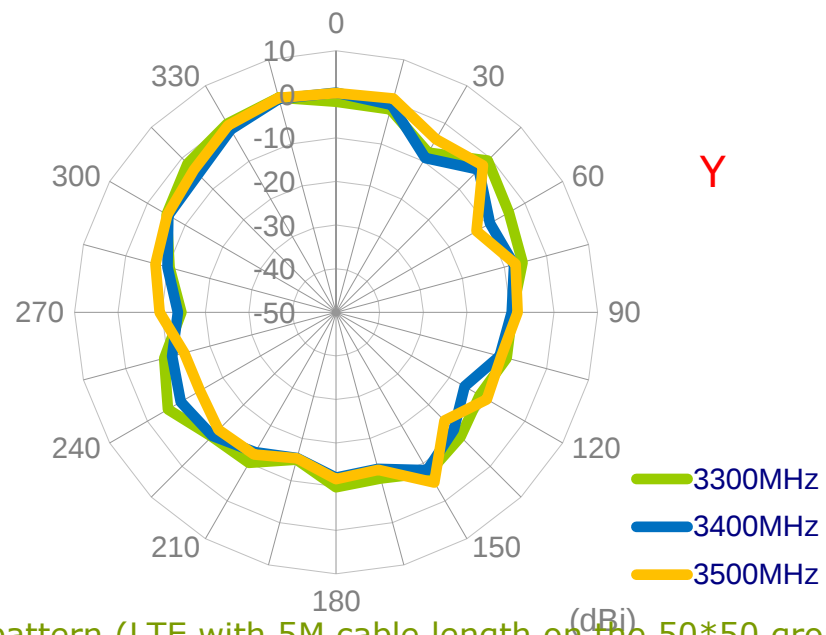
3.1.8 3D Radiation pattern (LTE with 5M cable length on the 50*50 ground plane)
