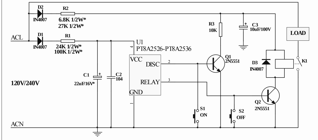
TO94 Universal Timer to drive RELAY with two buttons
