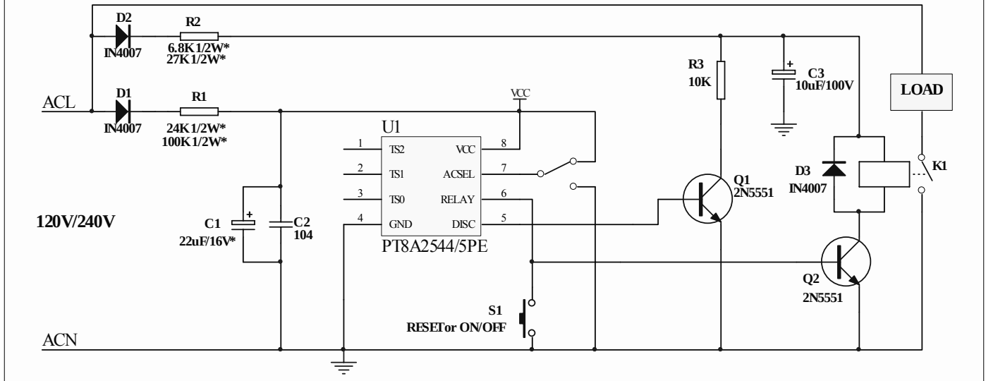
DIP8 Universal Timer to drive RELAY with one button
