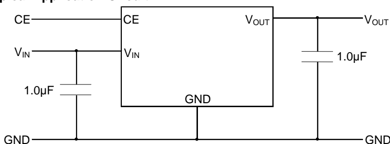
Figure 1. Application Circuit
