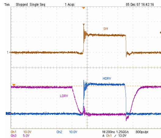
Fig. 7 Gate Signals at 25A Load
