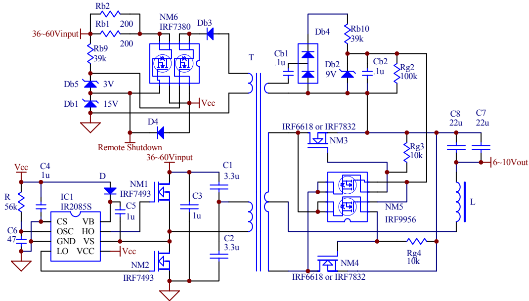
Fig. 2 Complete schematic of IRDC2085S-DF Demo Board
