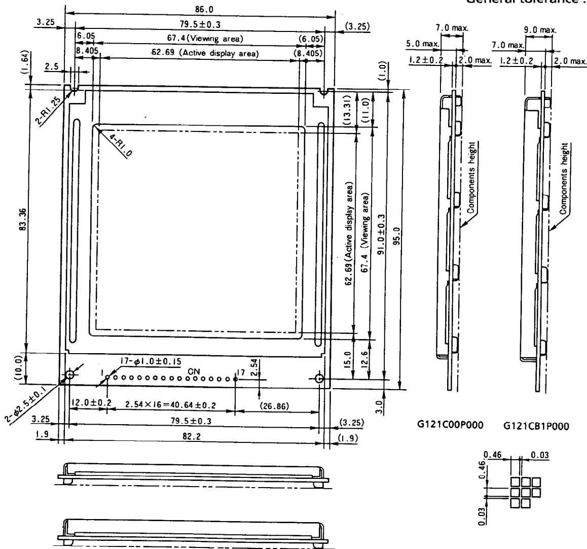
Figure 2 Dimensions
