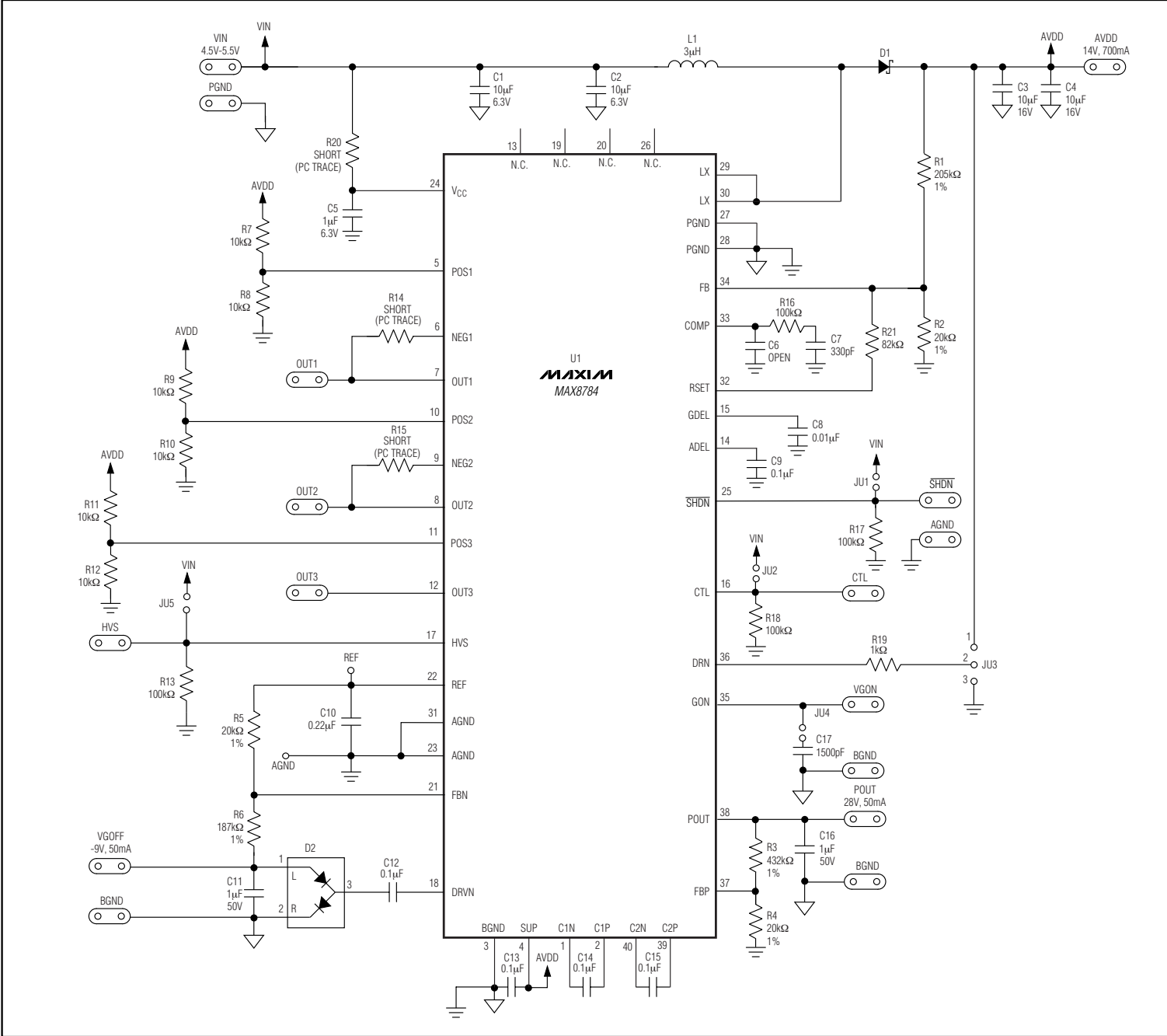
Figure 1. MAX8784 EV Kit Schematic
