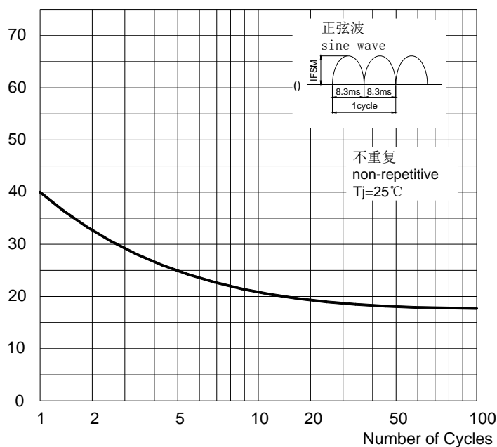
图2: 耐正向浪涌电流曲线 FIG2:Surge Forward Current Capadity
