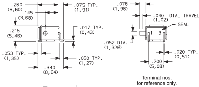
GP11MSABE SPST
