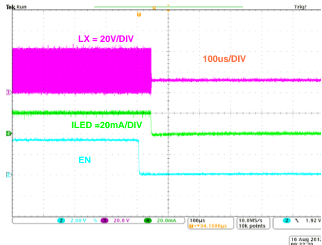
FIGURE 19. ISL97672B SHUTS DOWN AND STOPS SWITCHING ~30µs AFTER V_{EN} GOES LOW
