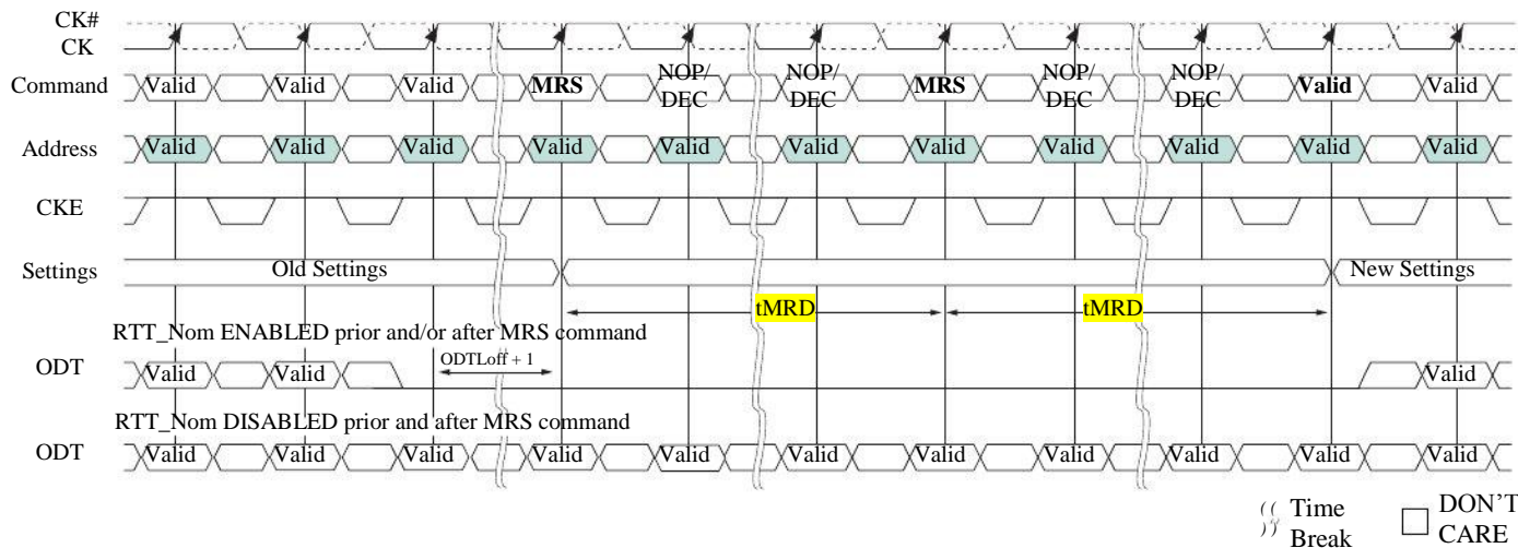
Figure 2.3.1a tMRD Timing
