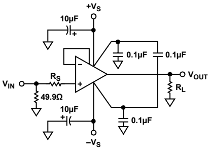
Figure 49. Noninverting Load Configuration
