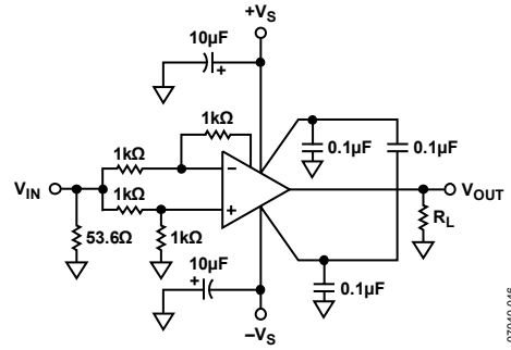
Figure 52. Common-Mode Rejection
