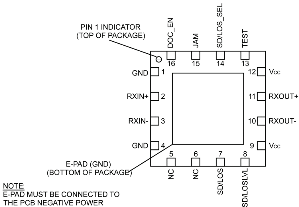
16-Pin 3mm × 3mm QFN (Top View)
