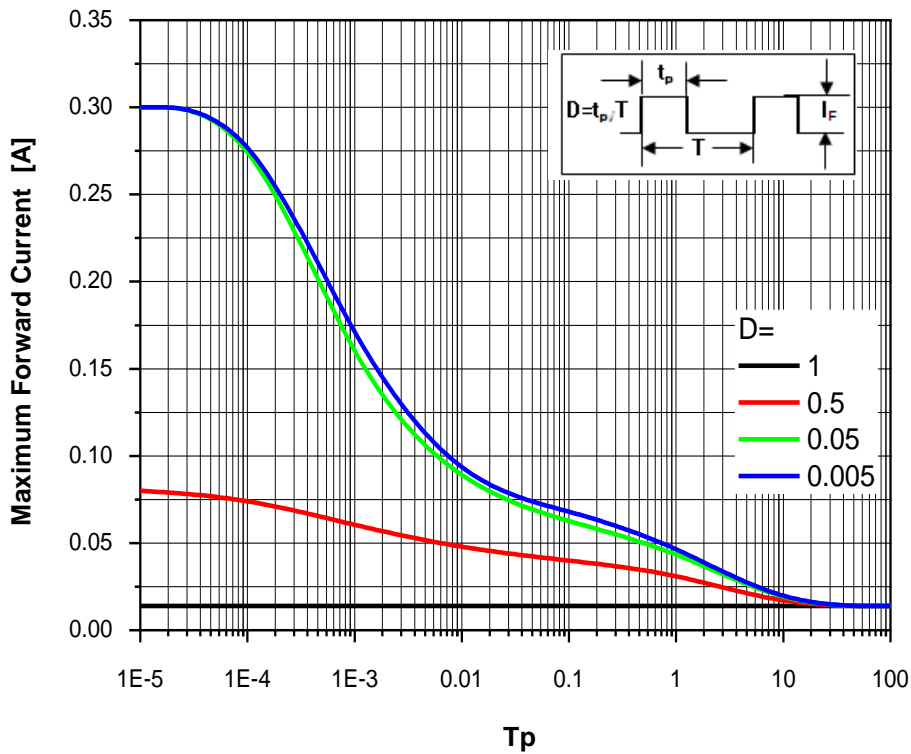
Fig 12. Maximum Forward Current vs. Duty Ratio, T_j = 85^\circ\text{C}
