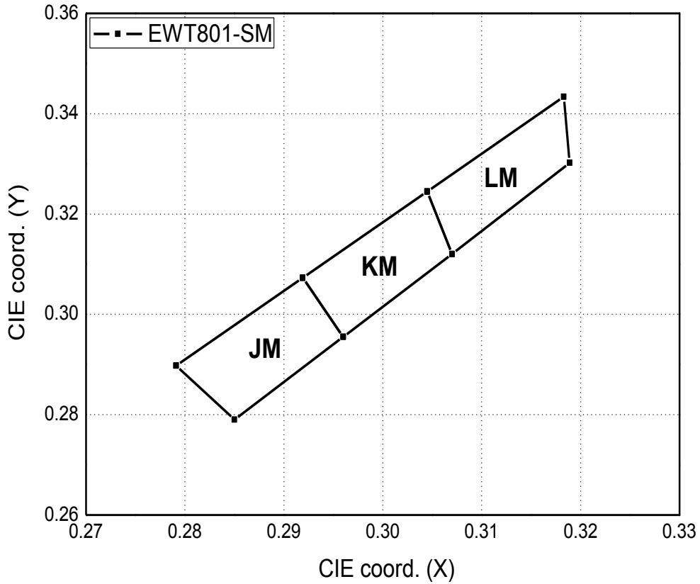
CIE Chromaticity Diagram, I_F = 20\text{mA} , T_j = 25^\circ\text{C}
