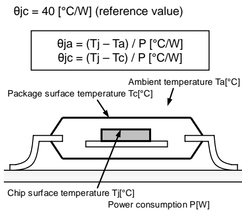
Fig.25 Thermal resistance
